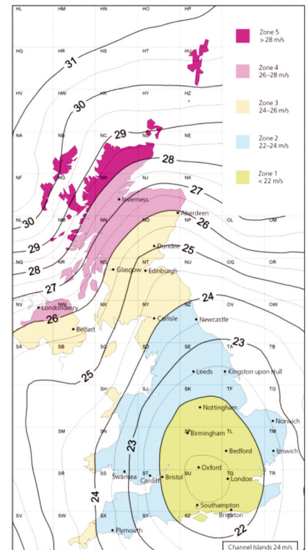
HIC®, reproduced with permission from BRE DG 489, 2014 edition.
